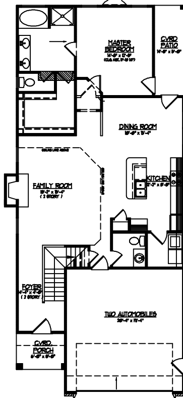
RE-C2088 First Floor Plan
