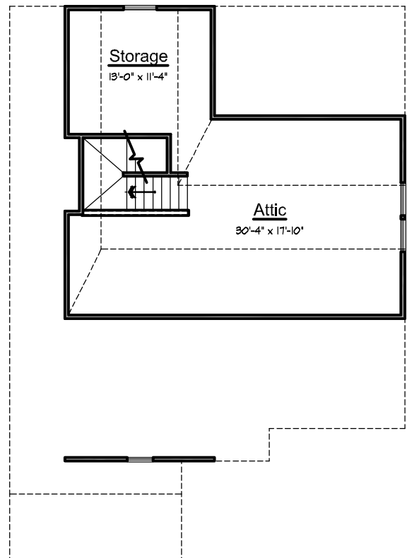
ATTIC FLOOR PLAN OPTIONAL FINISHED SQUARE FOOTAGE = 642
